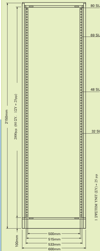
Front Elevation
